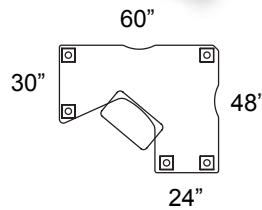
L-Desk with Adjustable Keyboard Tray H2WD244860 (L/R)
