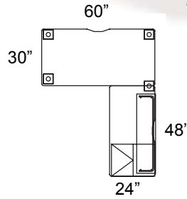
Desk with Return, Pedestal & Shelf H2WB3060
