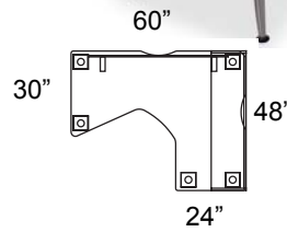
L-Desk with Hutch & Modesty Panel H2WF244860 (L/R)
